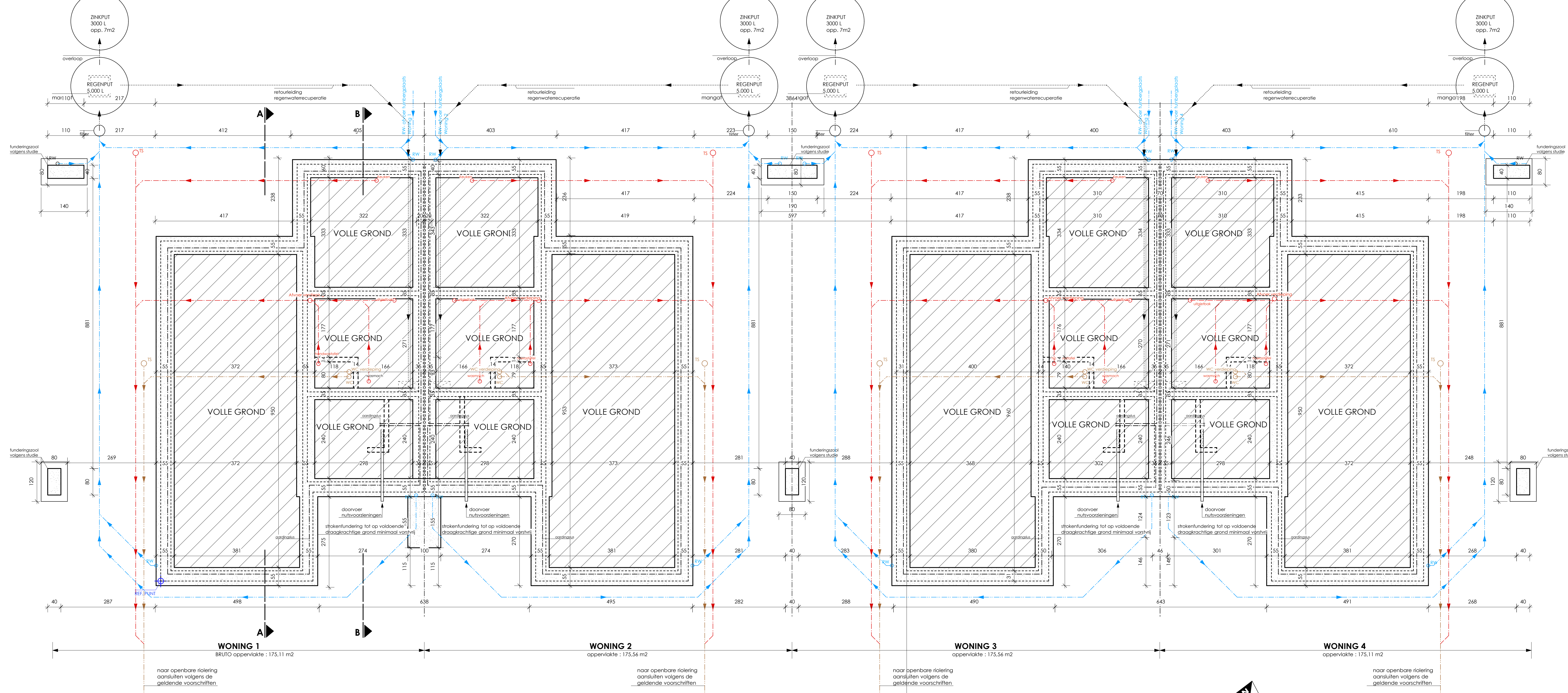
FUNDERINGS- & RIOLERINGSPLAN
